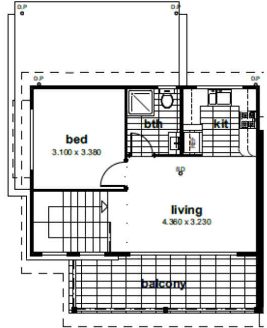
LEVEL 1 FLOOR PLAN
