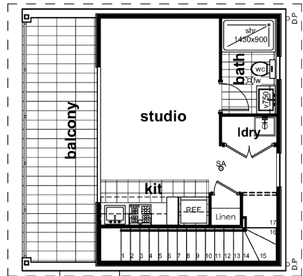
LEVEL 1 FLOOR PLAN
