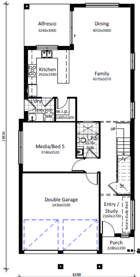
Ground Floor Scale 1 : 100
