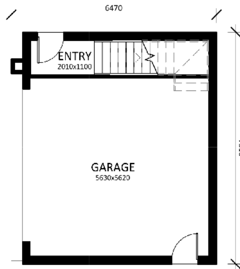
Studio Ground Floor Plan
