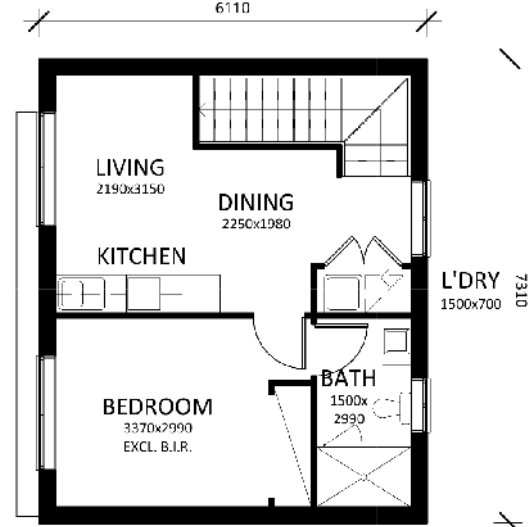
Studio First Floor Plan
