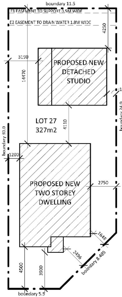
Site Plan
