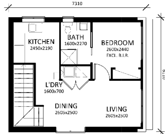
Studio First Floor Plan
