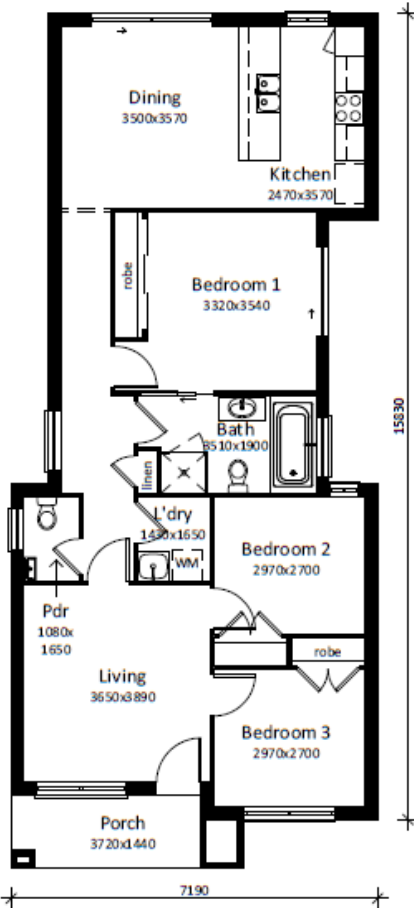
Floor Plan Scale 1:100
